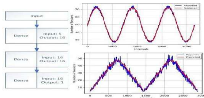
Figure 3. The predictions made by neural networks and the actual values about network density
