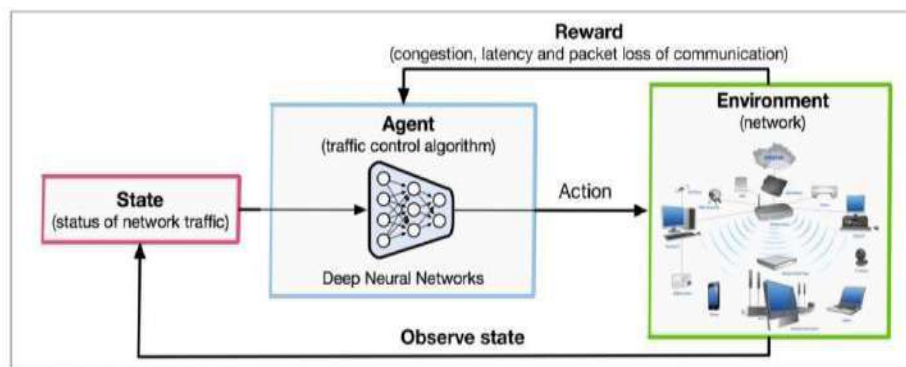
Figure 2 Representation of working process of an agent
