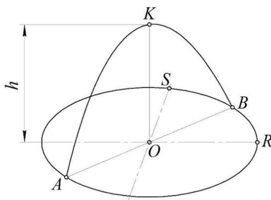
3-rasm. Elliptik reja asosida qobiq sirtini modellashtirishning geometrik sxemasi.
